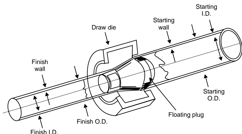
Fig. 19: Tube Drawing
