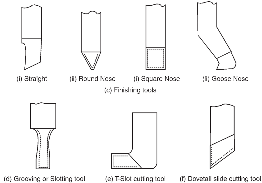
Fig. 6.16: Planer tools
