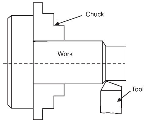
Fig. 6.3: Plain turning
