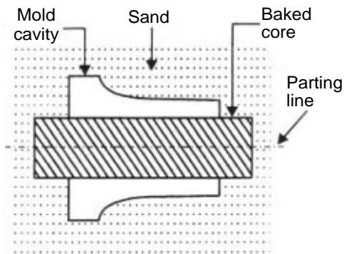
Fig. 21: Horizontal Core
