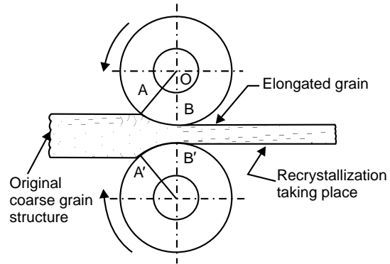
Fig. 17: Hot-rolling Process
