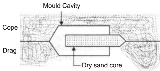
Fig. 22: Balanced Core
