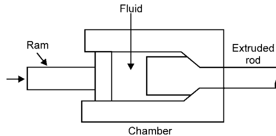
Fig. 4.23: Hydrostatic Extrusion
