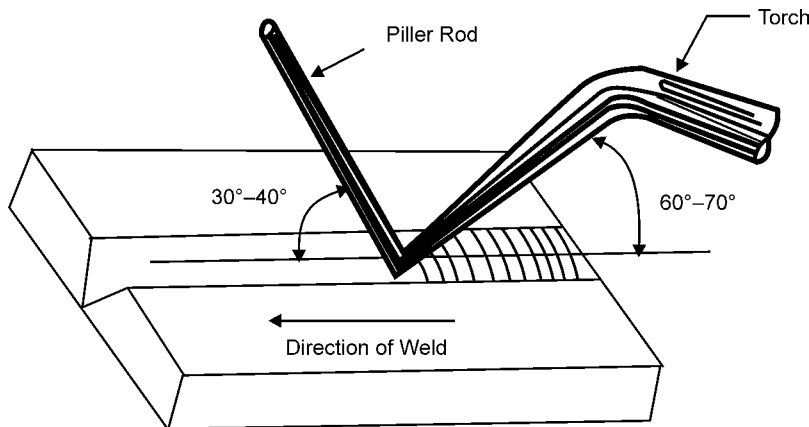
Fig. 7.4: Leftward Welding
